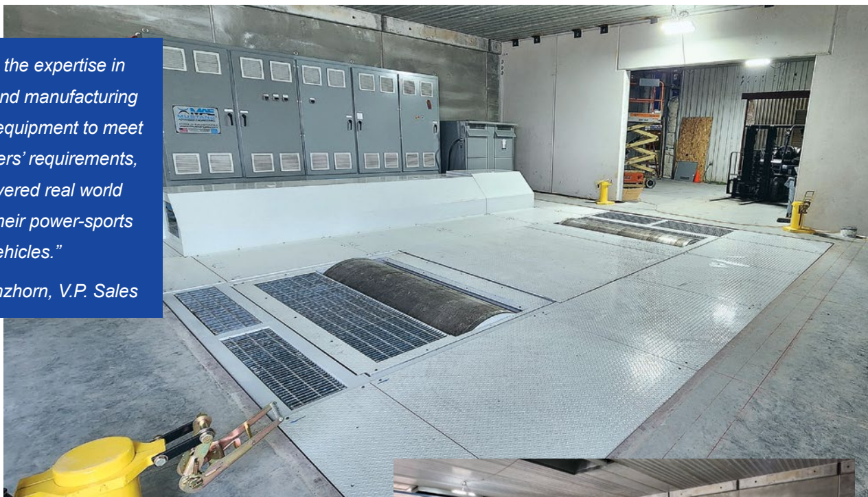
160,000 CFM, 250-hp frontal cooling fan system with speed/fan synchronization.
